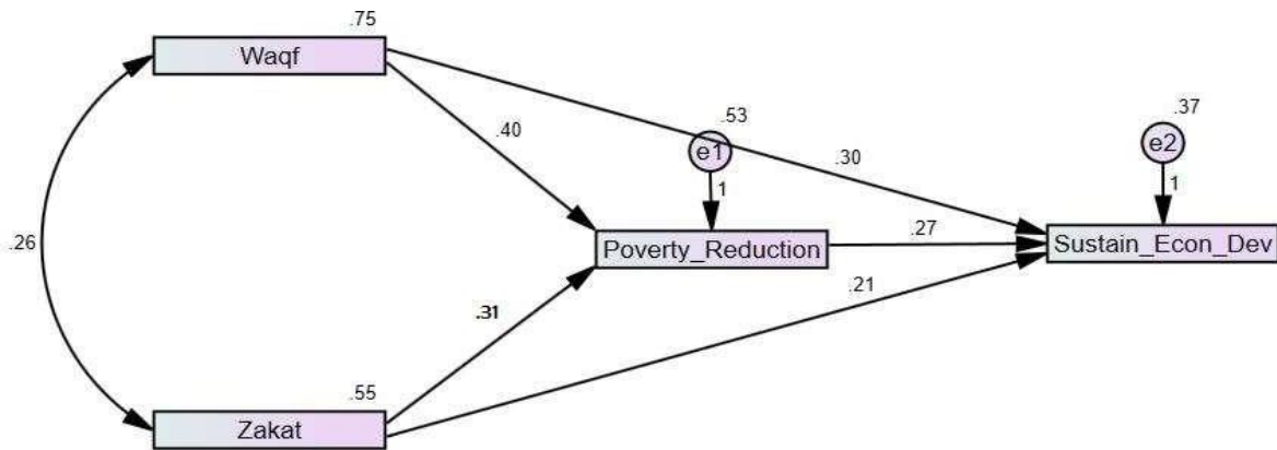
Figure 2: Measurement Model
